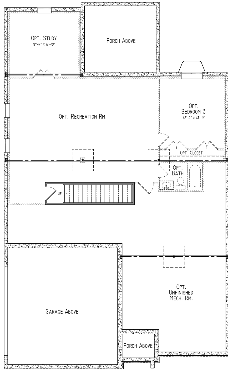
Foundation Plan
