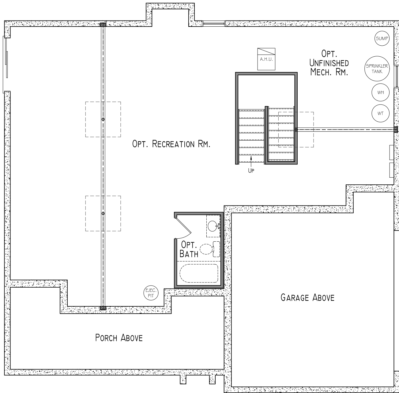
Foundation Plan
