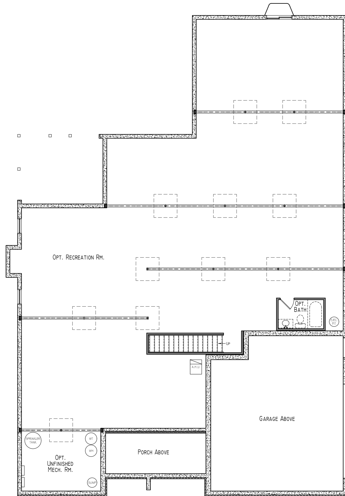
Foundation Plan
